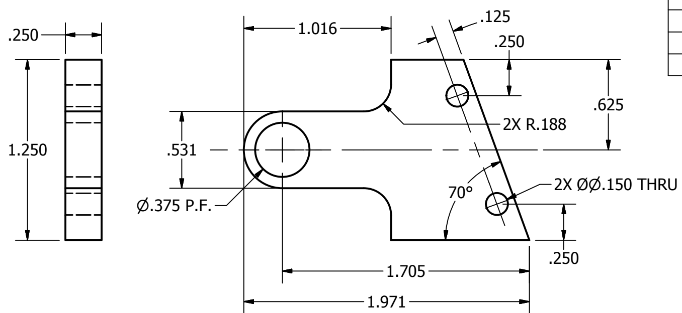
Bracket, Hall Effect Sensor
